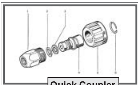
Quick Coupler
