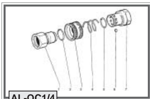
AL-QC1/4
